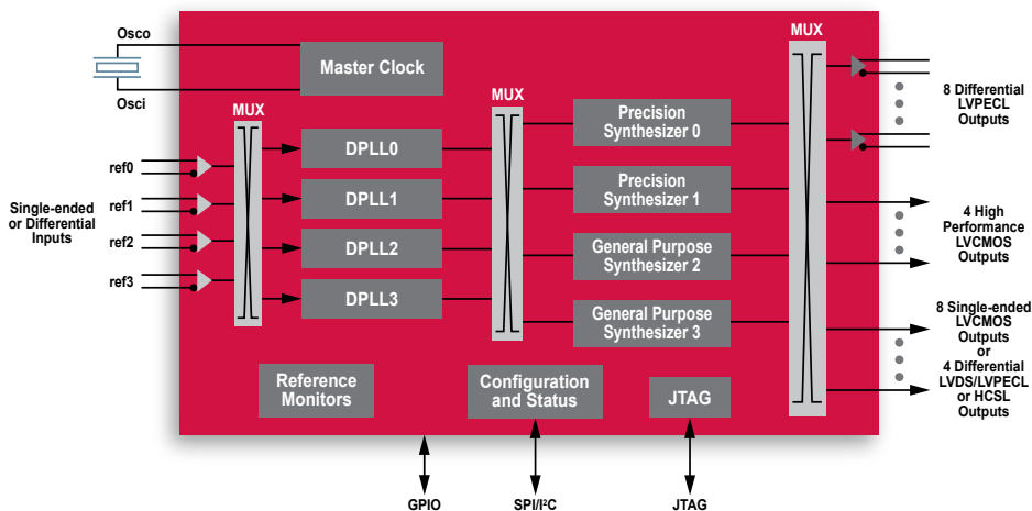
ZL30160 Block Diagram
